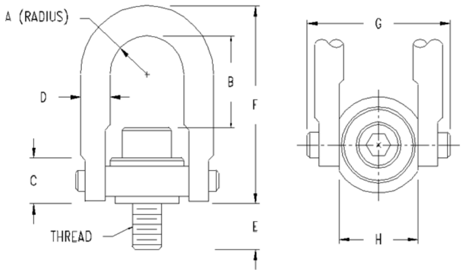
Safety Swivel Hoist Ring
